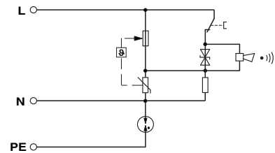
Circuit diagram
