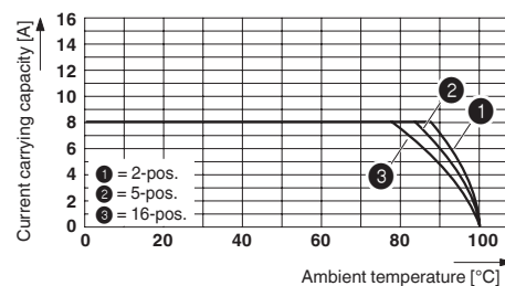
Type: PT 1,5/...-PVH-3,5 with PST 1,0/...-3,5
