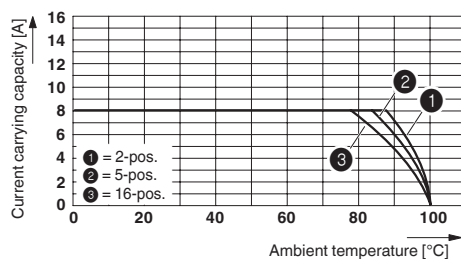
Type: PT 1,5/...-PH-3,5 with PST 1,0/...-3,5
