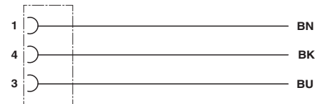
Contact assignment of M8 plugs/sockets
