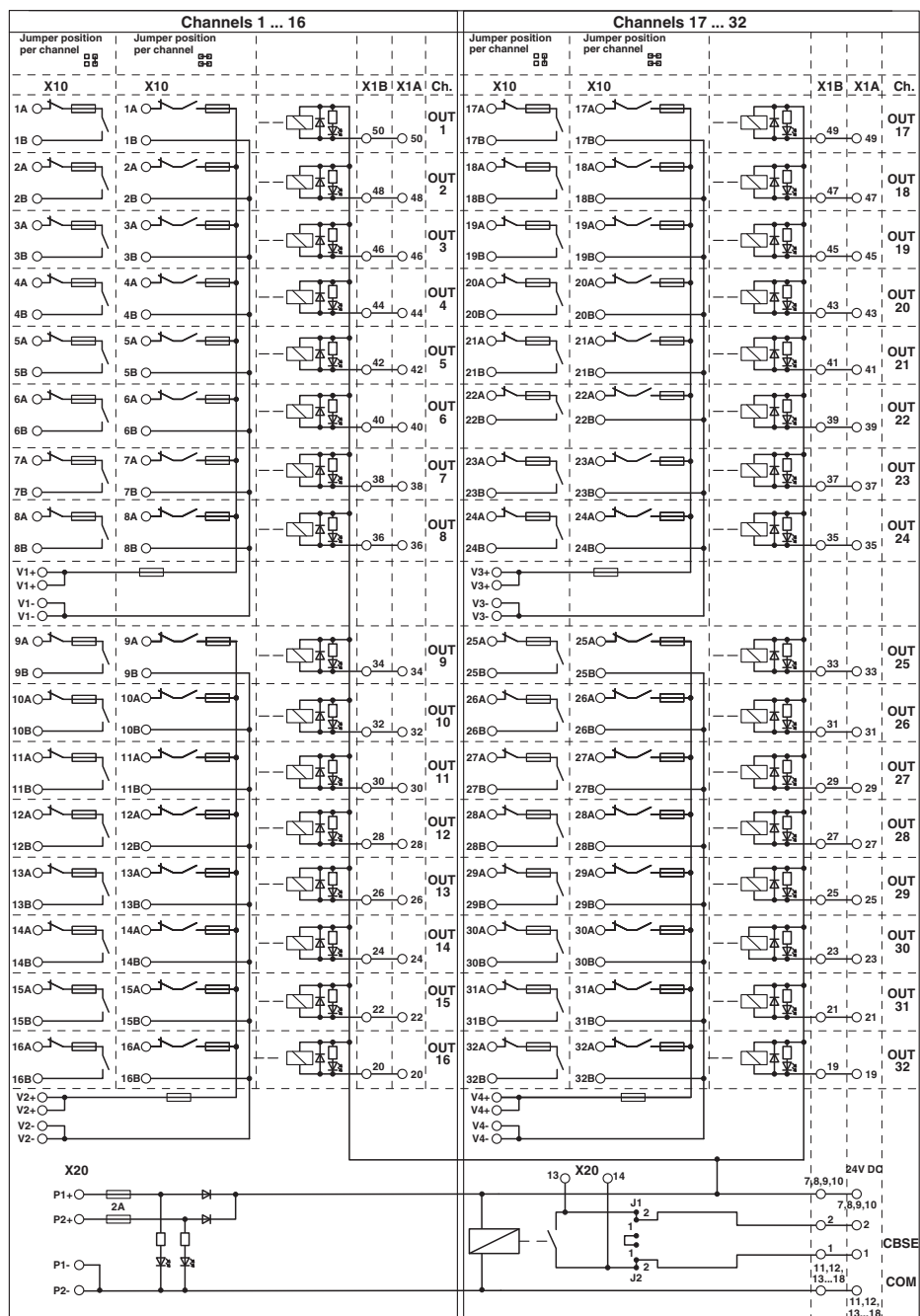
Circuit diagram
