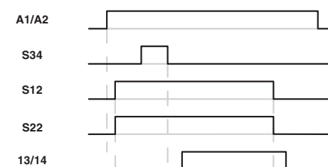
Figure 2 Time diagram PSR-MS35
