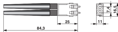
SCRJ connector IP20
