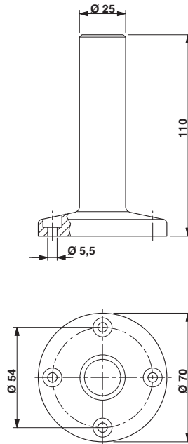
Dimensional drawing
