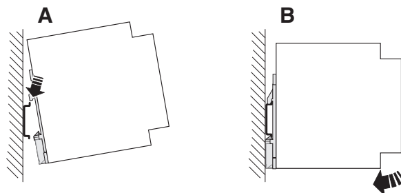
Figure 6 Assembly
