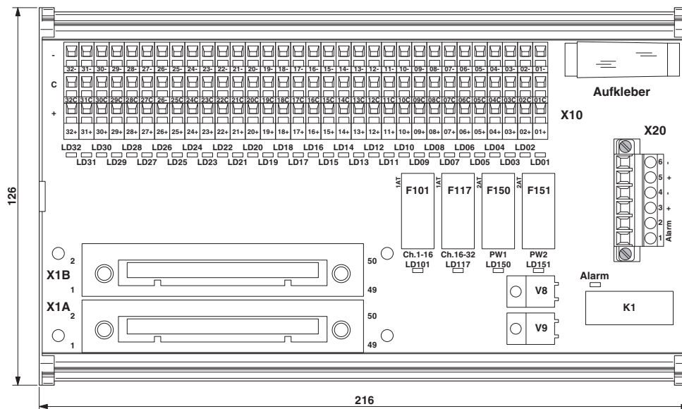
Dimensional drawing
