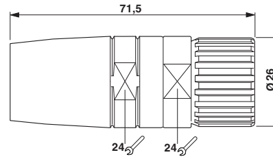
Dimensioned drawing
