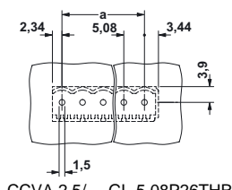
CCVA 2,5/...-GL-5,08P26THR
