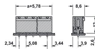
CCVA 2,5/...-GL-5,08P26THR
