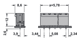
CCVA 2,5/...-GR-5,08P26THR
