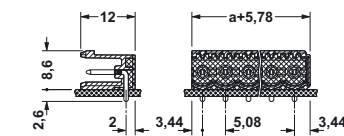
CCA 2,5/...-GR-5,08P26THR
