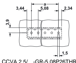
CCVA 2,5/...-GR-5,08P26THR
