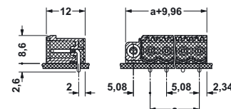
CC 2,5/...-GFL-5,08P26THR
