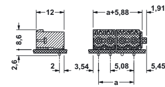
CCA 2,5/...-GR-5,08RNP26THR
