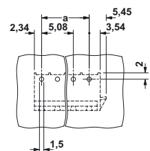
CCA 2,5/...-GR-5,08RNP26THR
