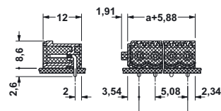
CCA 2,5/...-GL-5,08RNP26THR
