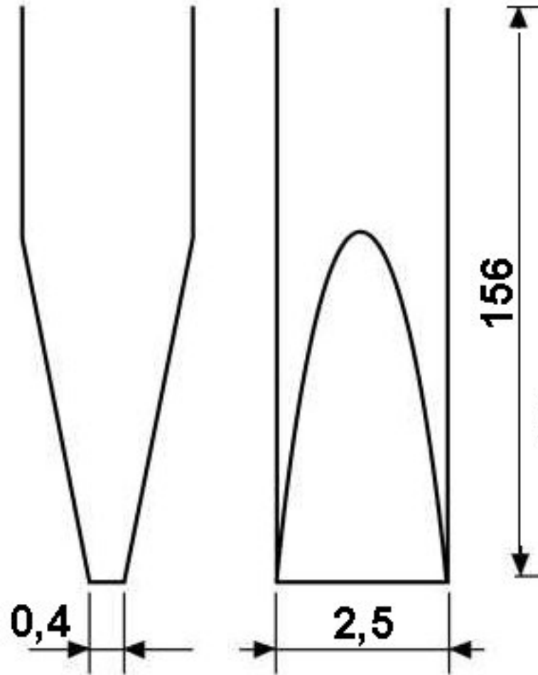
Dimensioned drawing
