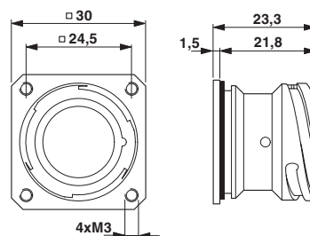
Dimensional drawing
