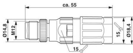
Dimensioned drawing
