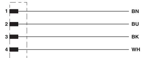
Contact assignment of the DEUTSCH DT04-4P
