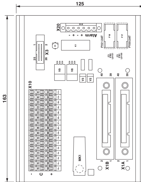
Dimensional drawing
