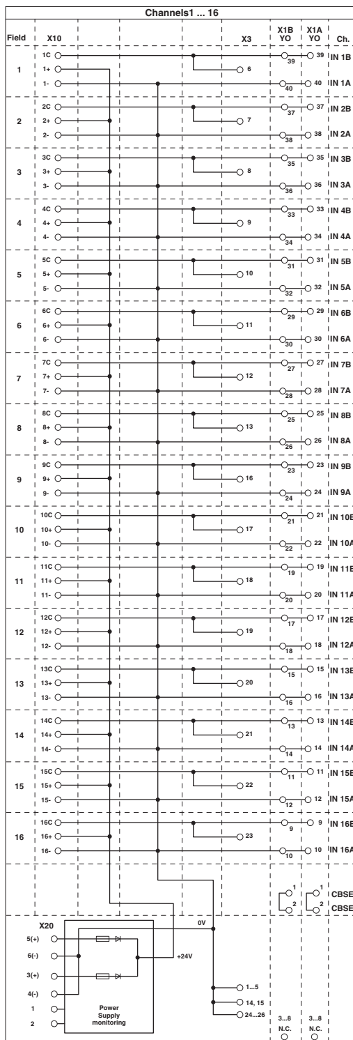
Circuit diagram
