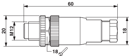
Dimensional drawing
