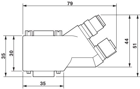
Figure 3 Dimensions, angled 35°
