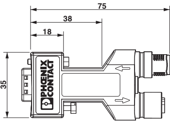
Figure 4 Dimensions, axial
