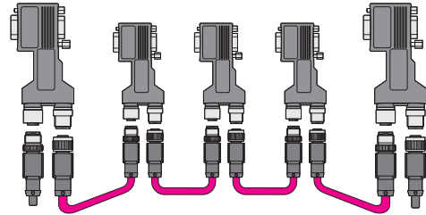
Figure 12 Connecting
