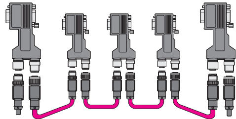
Figure 8 Connecting
