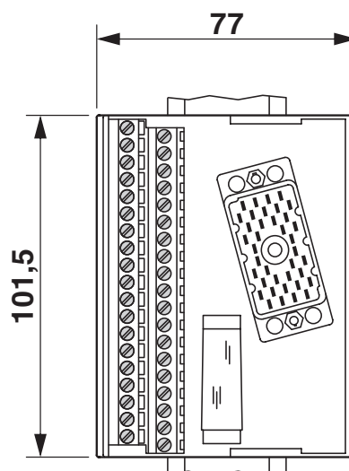
Dimensional drawing
