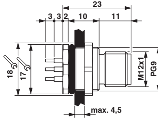
Dimensioned drawing
