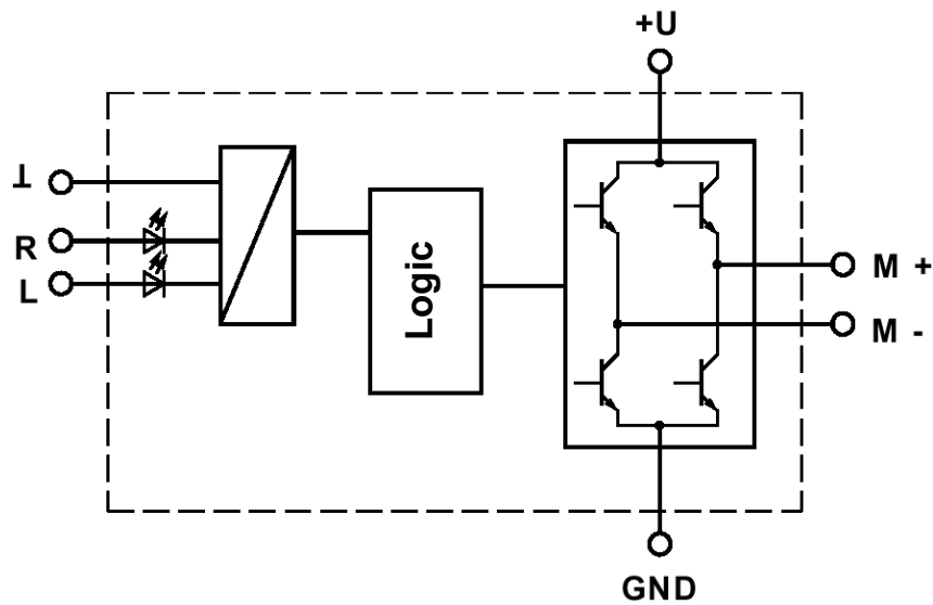
Figure 3 Block diagram
