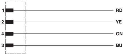
Contact assignment of the M8 plug
