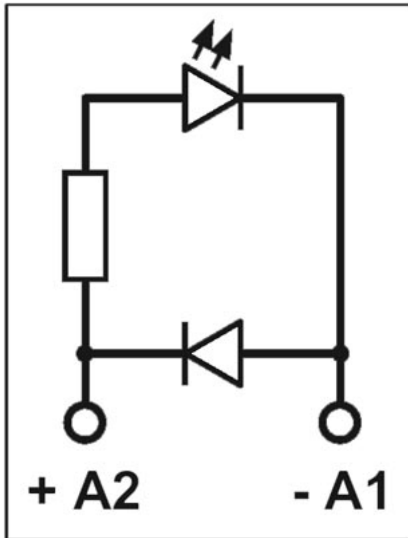
Circuit diagram
