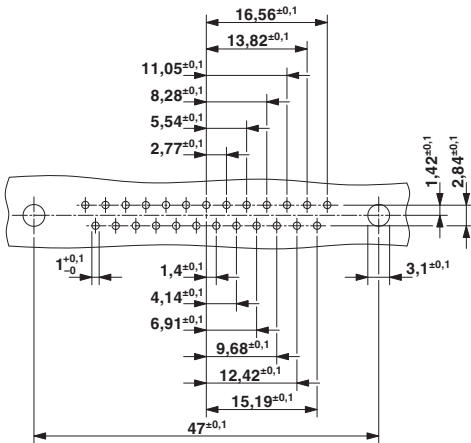
Drilling diagram
