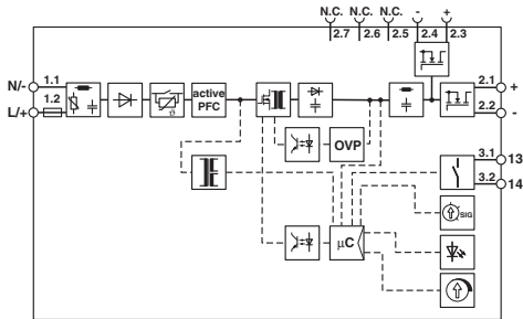
Block diagram
