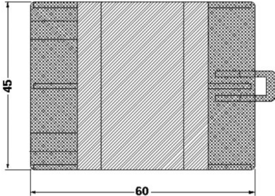
Dimensioned drawing
