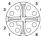
Assignment of the LAN female connector
