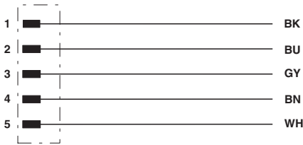
Contact assignment of 7/8" plug
