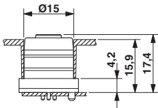
Dimensional drawing
