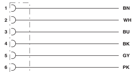
Contact assignment of M8 socket
