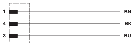
Contact assignment of the M12 plugs
