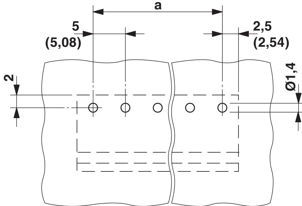
Drilling diagram
