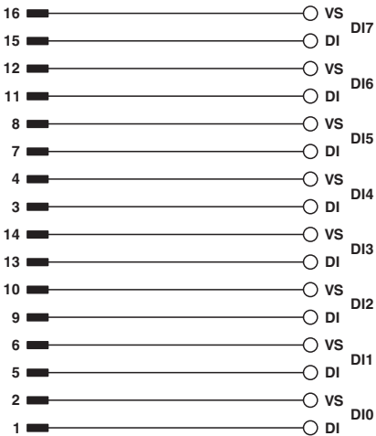
Circuit diagram
