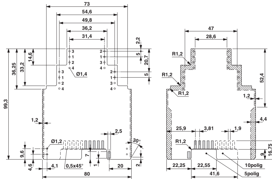
Dimensioned drawing
