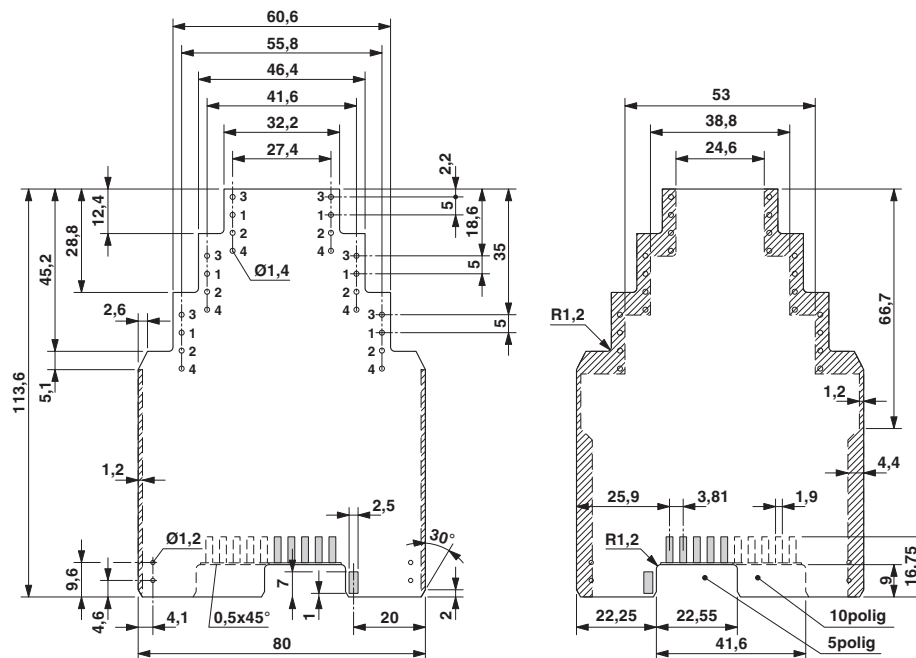
Dimensioned drawing
