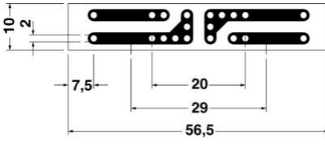
Dimensioned drawing
