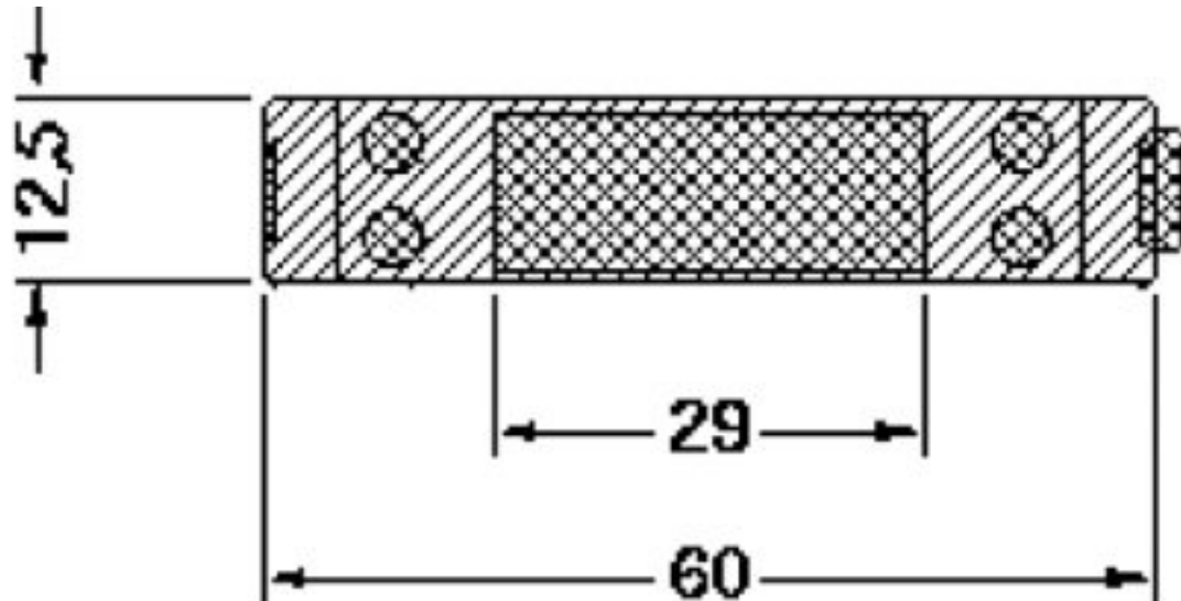
Dimensioned drawing
