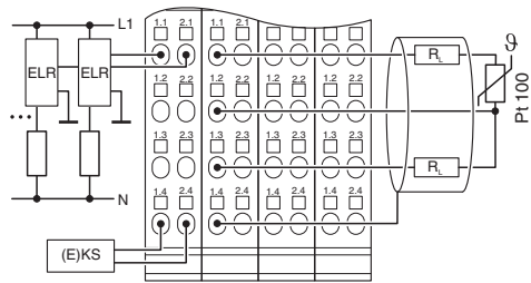
Connection diagram
