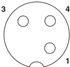
Pin assignment M12 socket, 3-pos.
