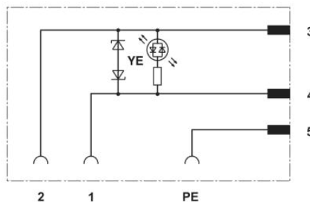
Circuit diagram
