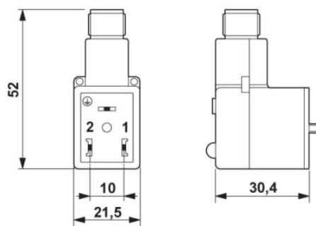
Dimensioned drawing
