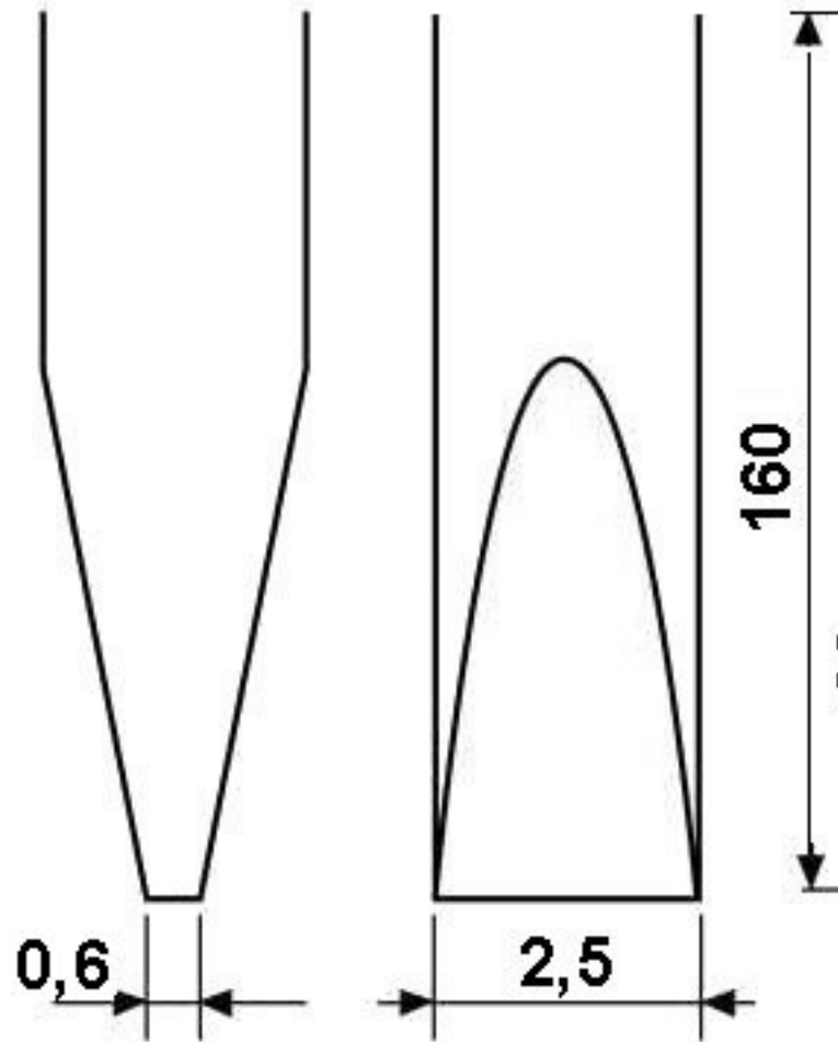
Dimensioned drawing
