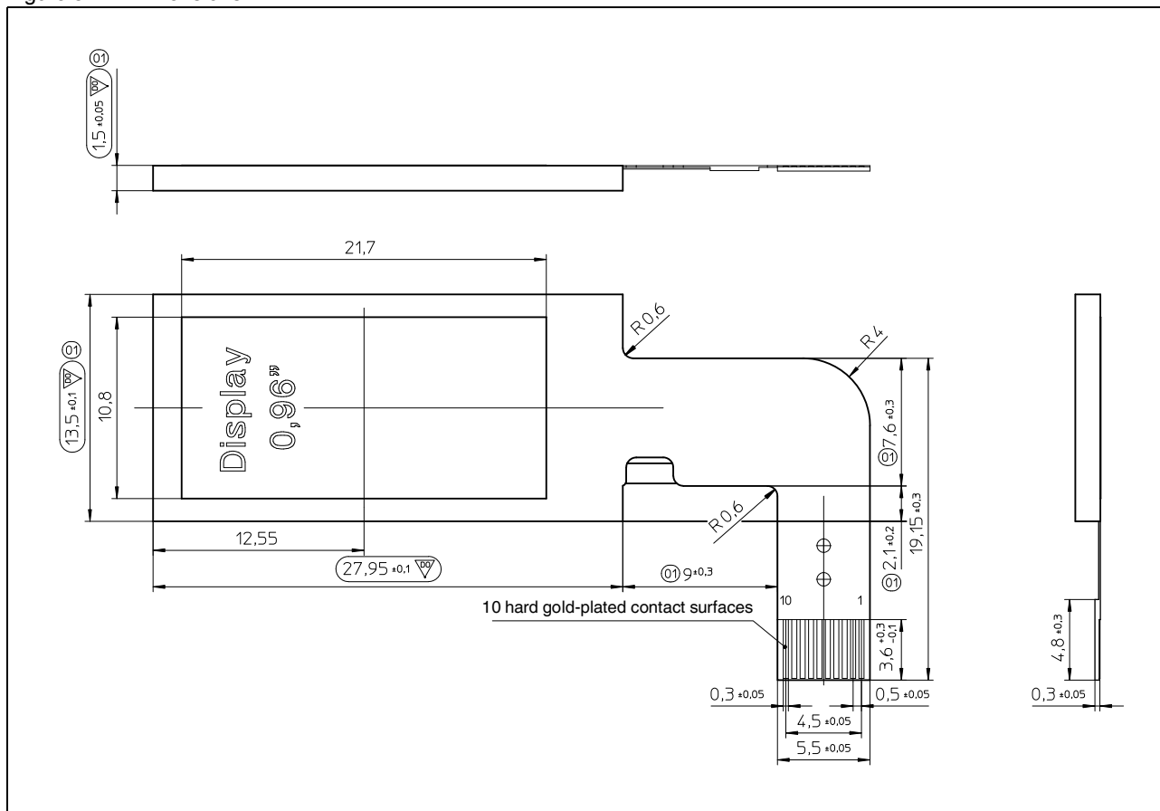
Figure 8 Dimensions
