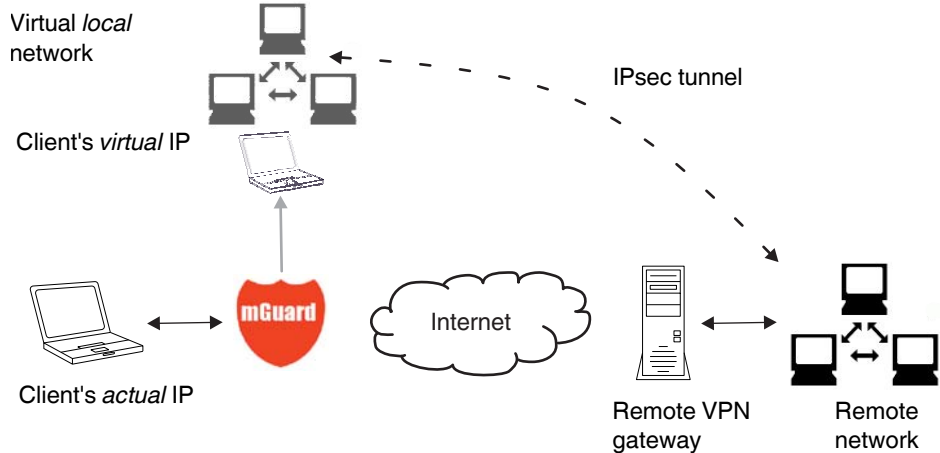
Figure 5-4 Virtual IP
