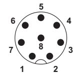
Pin assignment M12 plug, 8-pos., view plug side
