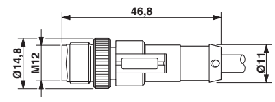
Dimensional drawing
