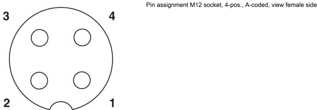
Schematic diagram
