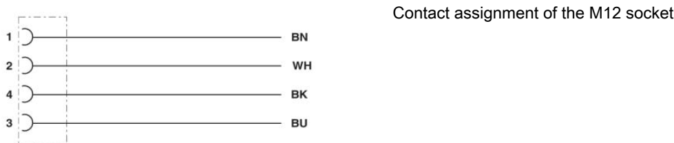
Circuit diagram
