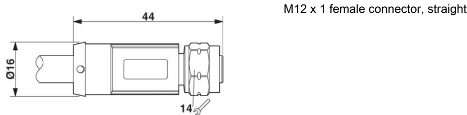
Dimensioned drawing
