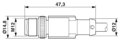
Dimensioned drawing
