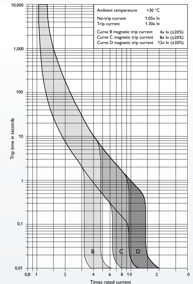
Magnetic tripping currents are increased by 30% on DC supplies
