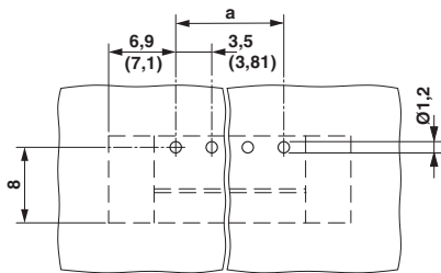
Drilling diagram
