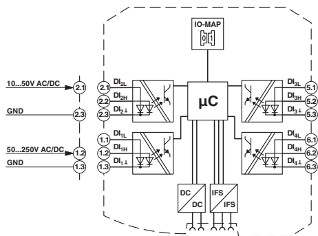
Block diagram
