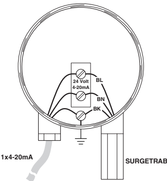
Application drawing
