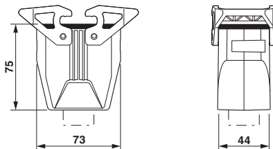
Dimensional drawing
