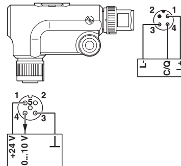
Figure 5 Connection example
